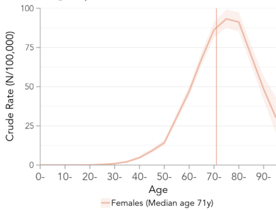
Age-specific incidence, 2018-2022
