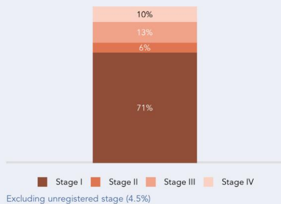
Stage distribution
